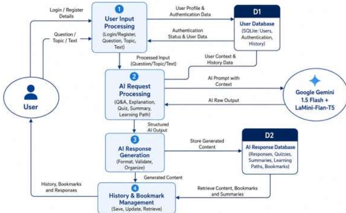
Level-1 Data Flow Diagram (DFD)
